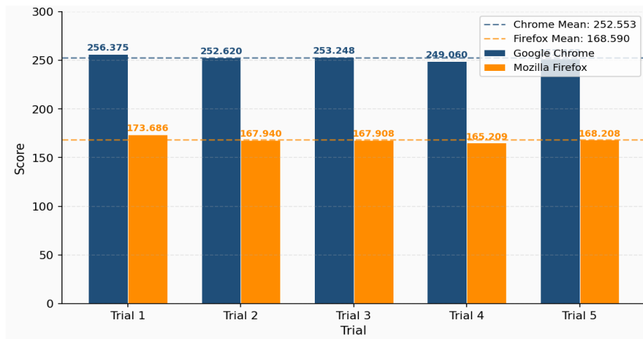
Figure 2. JetStream 2.0 Per-Trial Score Comparison
