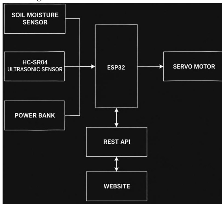
Figure 1. Smart Trash Bin System Block Diagram
