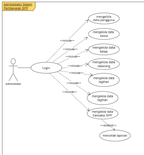
Figure 1 Administrator Use Case Diagram
